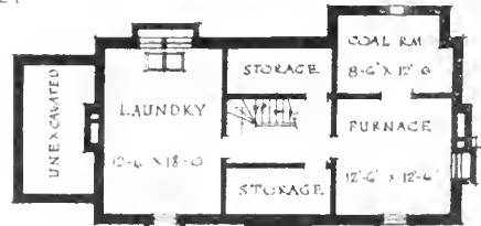
BASEMENT PLAN
